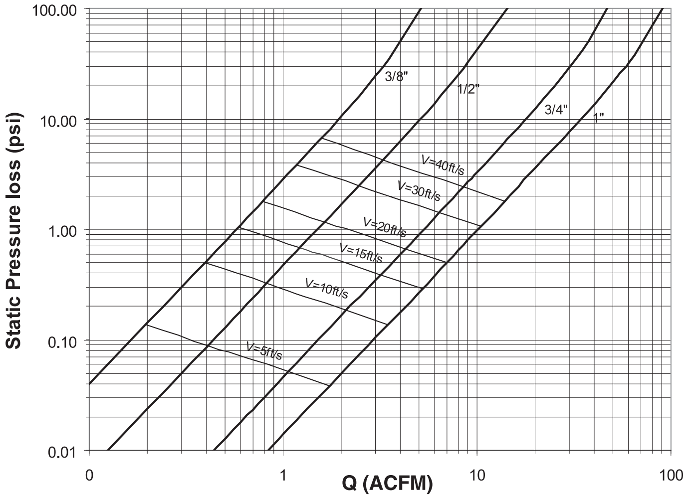
Pressure Loss through Duratec Fittings in Equivalent Feet of Pipe
