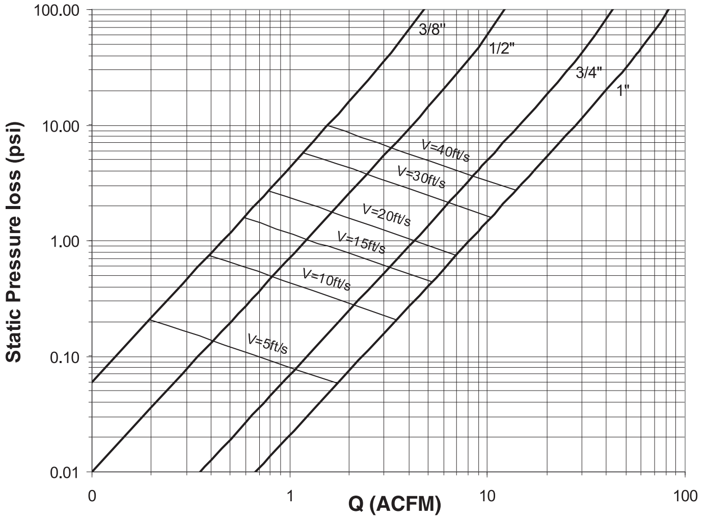
Pressure Loss through Duratec Fittings in Equivalent Feet of Pipe
